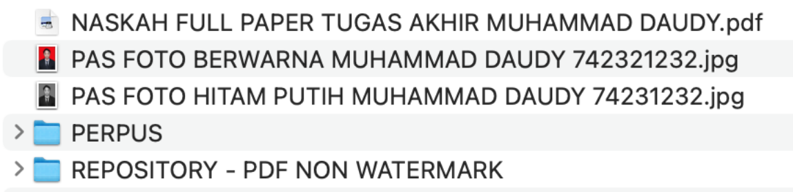
Gambar 2. Softfile CD/DVD
